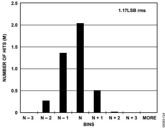
Figure 24. AD9434-370 Grounded Input Histogram; 370 MSPS
