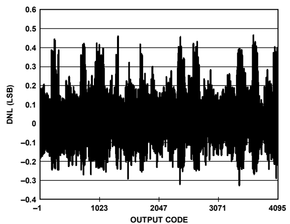
Figure 23. AD9434-500 DNL; 500 MSPS
